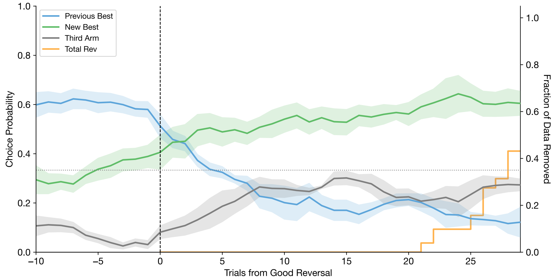
Good Reversal-Aligned Choices (mean \pm se across subjects | n=5 subjects, n=51 reversals)
